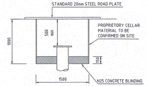
WELL PAD CELLAR (PLACE AT ALL WELL POSITIONS) SECTION B NTS
